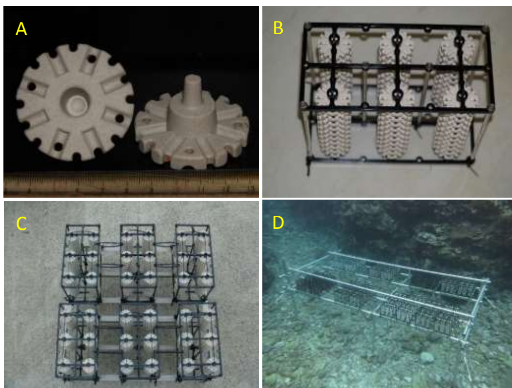
Figure 1. Coral Settlement Device. Ten devices were stacked into one batch. Six batches were arranged in a plastic frame. Six frames were set on a stainless steel platform. Eight platforms were deployed on a steel pipe stand placed on the sea bottom. A: coral settlement device, B: plastic frame, C: stainless platform, D: steel frame.
